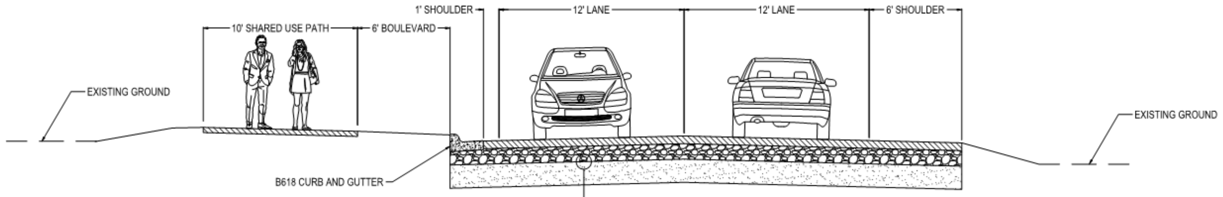
TYPICAL SECTION FOR NORTHERN PORTION OF PINEVIEW LANE NORTH
